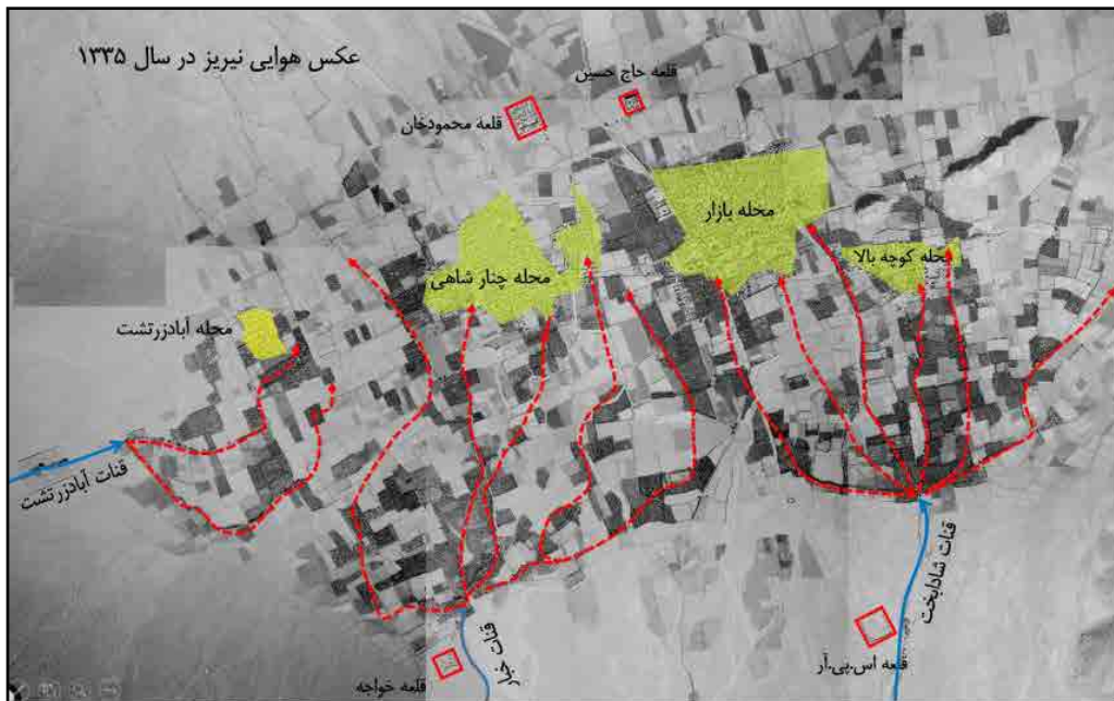
Fig. 11: The route of the Shadabakht, Khoabar, and Abadzardasht qanats that reach the neighborhoods of Neyriz City after irrigating gardens and fields (Authors, 2017).
