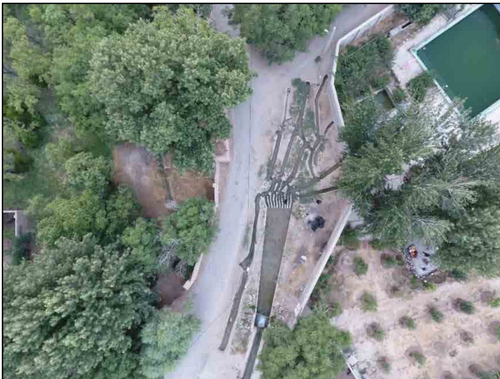
Fig. 12: Divider of Khoabar Qanat (Authors, 2017).
